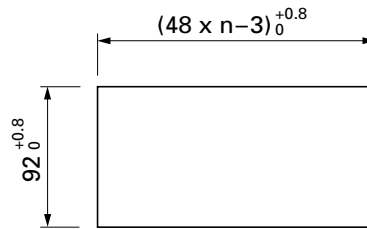
Side stick mounting (n units) (water-proof property is lost in this case)
