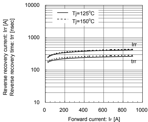
Reverse Recovery Characteristics (typ.) V_{CC}=600V , V_{GE}=\pm 15V , R_g=0.52\Omega , T_J=125^\circ C , 150^\circ C
