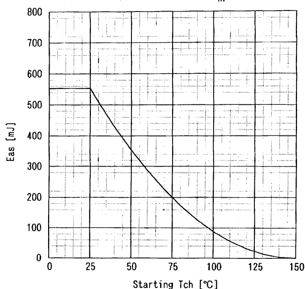
Maximum Avalanche energy vs. starting T_{ch} E_{as} = f(\text{starting } T_{ch}) : V_{CC} = 24V, I_{AV} \leq 70A , single pulse
