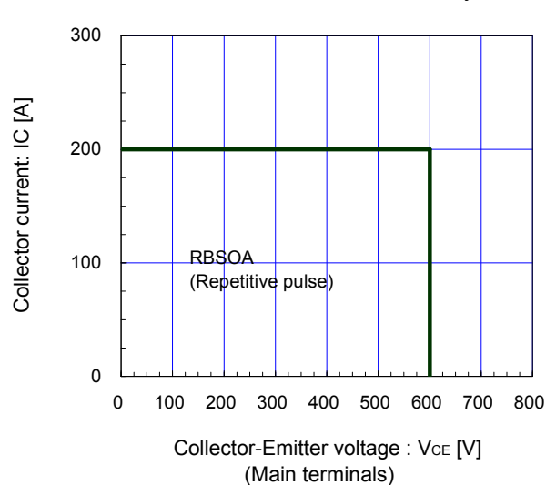
[ Inverter ]
