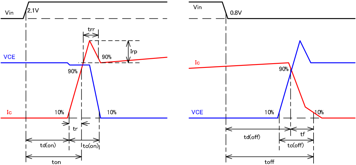
Fig.2-1: Switching waveforms
