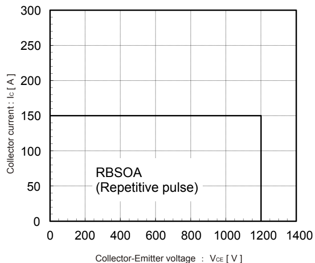
Reversed biased safe operating area V_{CC}=15V, T_J \leq 125^{\circ}C
