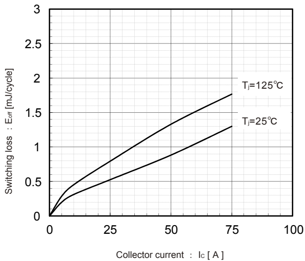
Switching Loss vs. Collector Current (typ.) V_{DC}=300V, V_{CE}=15V
