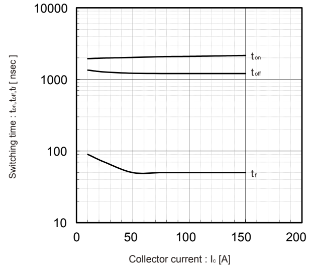
Switching time vs. Collector current (typ.) V_{DC}=300V , V_{CE}=15V , T_J=125^\circ C
