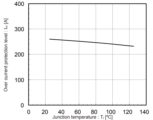
Over current protection vs. Junction temperature (typ.) V_{CE}=15V
