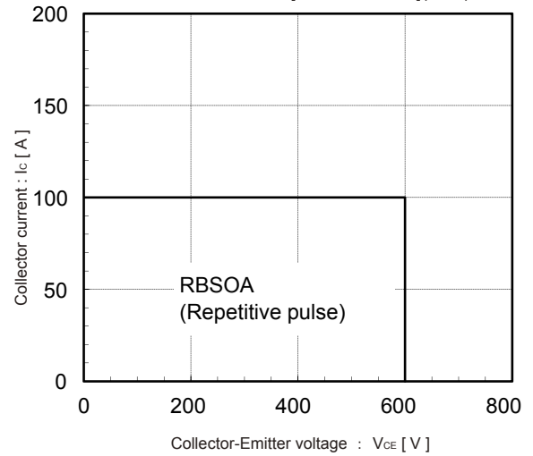
Reversed biased safe operating area V_{CE}=15V, T_J \leq 125^\circ\text{C} [Main Terminal] (min.)
