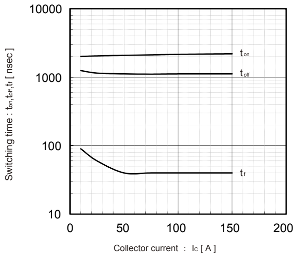
Switching time vs. Collector current (typ.) V_{DC}=300V , V_{CE}=15V , T_J=25^\circ C
