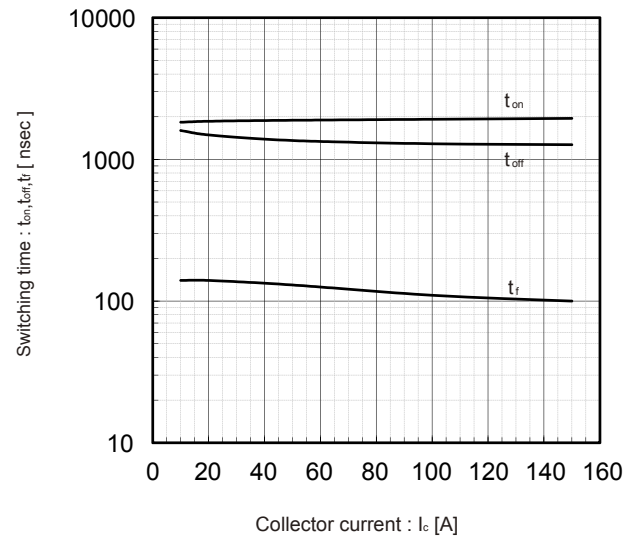
Switching time vs. Collector current (typ.) V_{DC}=600V , V_{ce}=15V , T_J=125^\circ C
