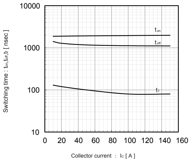
Switching time vs. Collector current (typ.) V_{DC}=600V , V_{ce}=15V , T_J=25^\circ C
