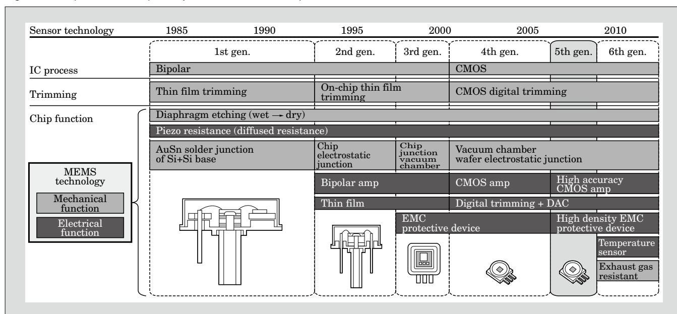
Fig.2 Development roadmap of Fuji Electric's automotive pressure sensors
