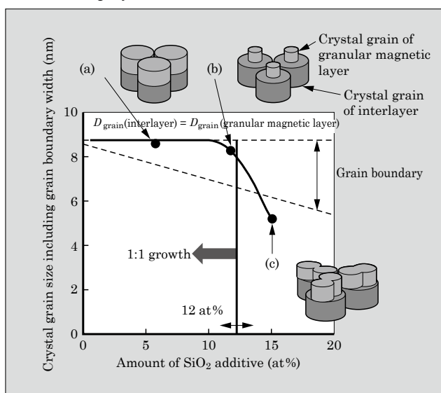
Fig.3 Schematic diagram of change in grain size and layer structure of CoPtCr-SiO 2 perpendicular magnetic recording layer
