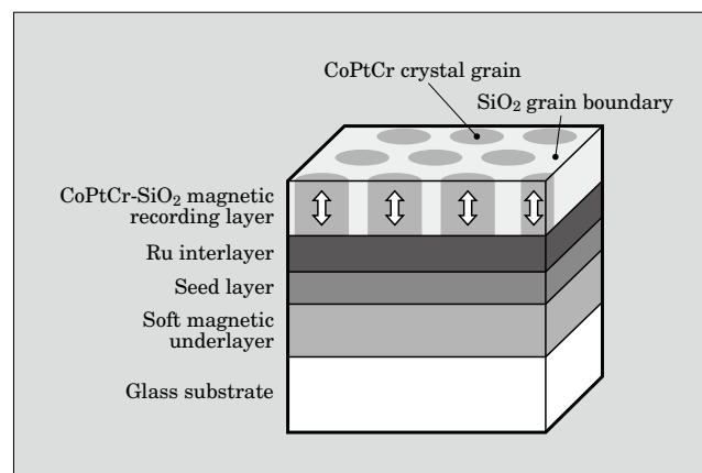
Fig.1 Layer structure of CoPtCr- SiO 2 perpendicular magnetic recording media with glass substrate
