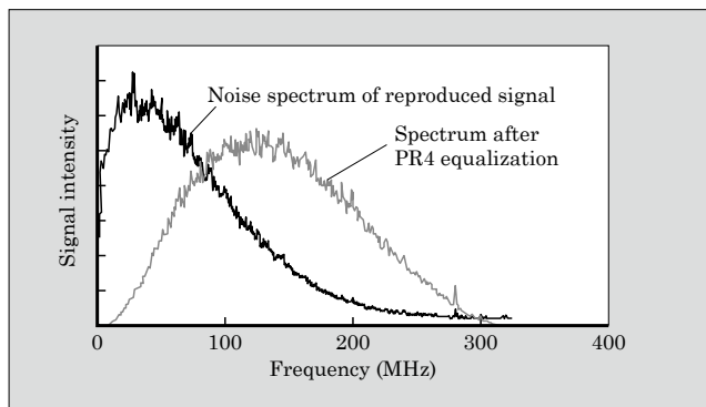
Fig.8 Noise spectrum after multiplication by PR4-equalized filter
