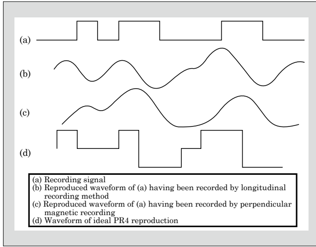
Fig.6 Examples of reproduced signal waveforms of a recorded signal
