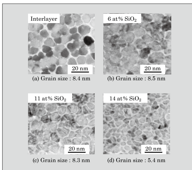
Fig.2 Cross-sectional TEM images of CoPtCr-SiO 2 perpendicular magnetic recording layers
