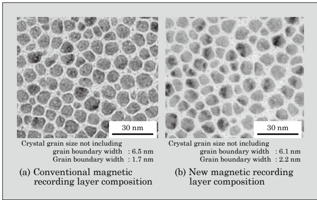
Fig.5 Cross-sectional TEM images of CoPtCr-SiO 2 perpendicular magnetic recording layers
