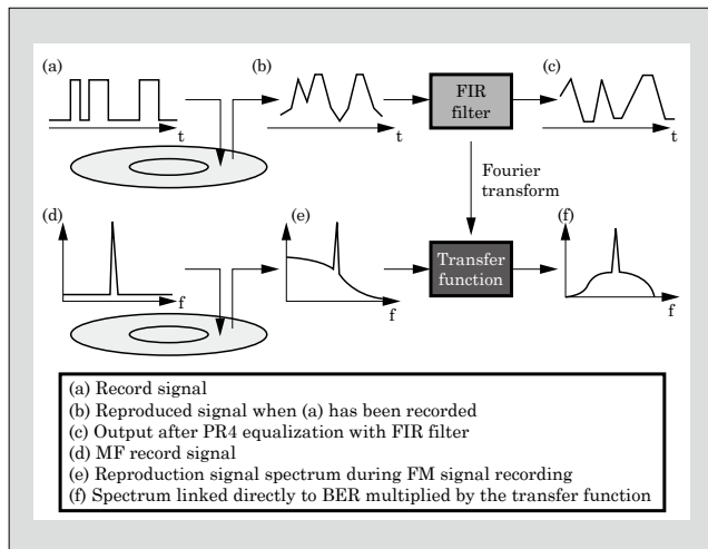
Fig.7 Signal processing steps with perpendicular magnetic recording
