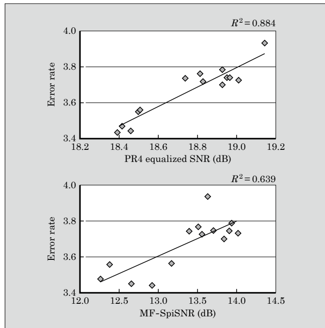
Fig.9 Relationship between each SNR and measured error rate
