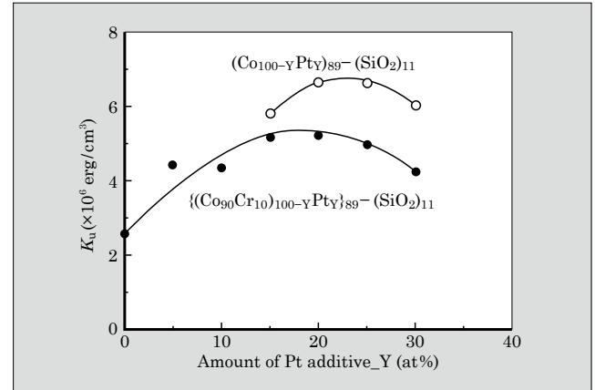
Fig.4 Change in K_u value according to amount of Pt additive in CoPtCr-SiO 2 perpendicular magnetic recording media
