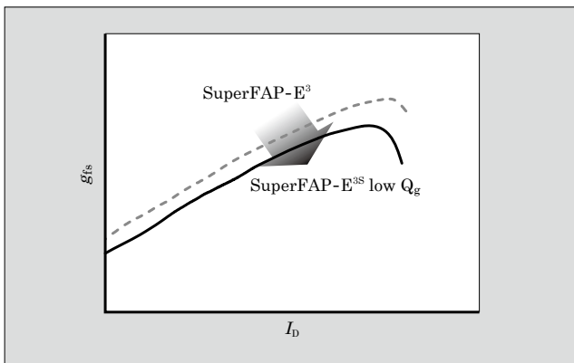
Fig.4 g_{fs} comparison
