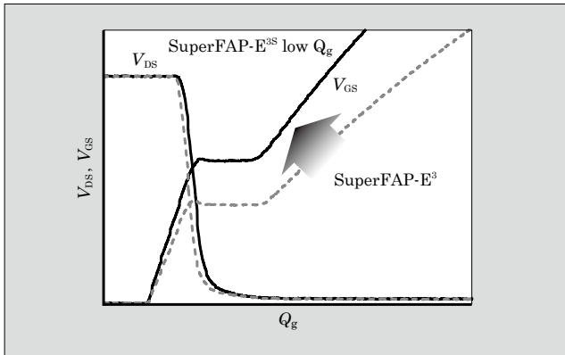
Fig.3 Q_g comparison
