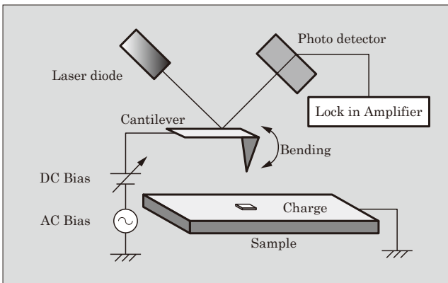
Fig.10 Principle of EFM Measurement
