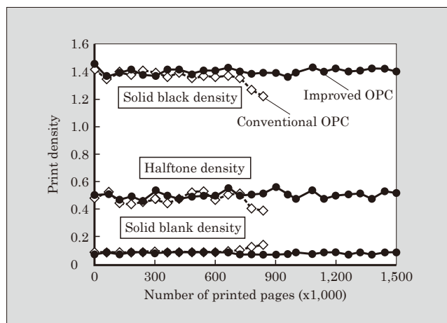
Fig.5 Printing Characteristics (Print Density) of Photoconductors for Digital Copiers
