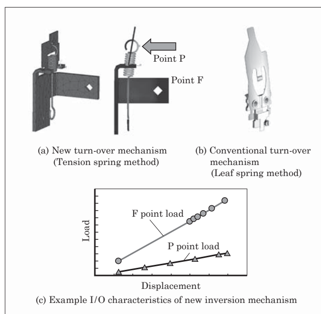
Fig.3 Turn-over mechanism
