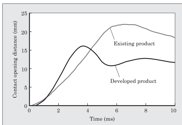
Fig.9 Comparison of contact opening characteristics
