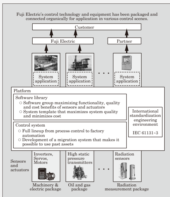
Fig.2 Control system platform
