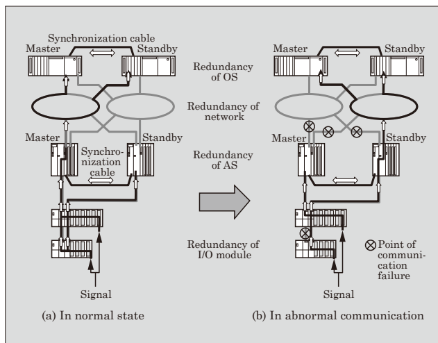
Fig.2 Concept of system switching by complete redundancy
