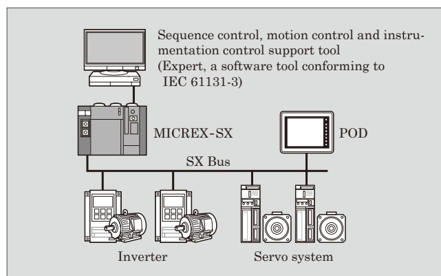
Fig.2 High-speed bus direct-connection system
