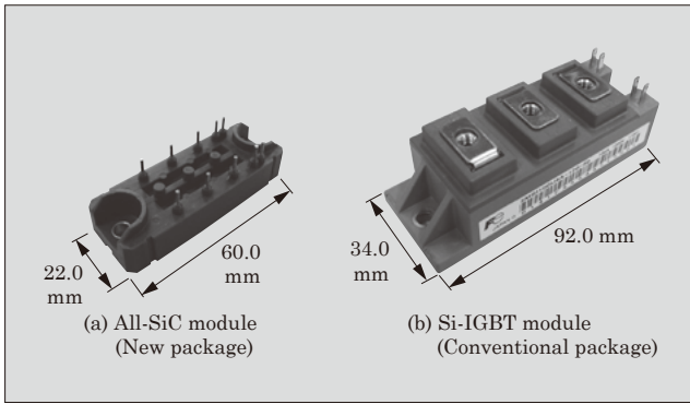
Fig.2 Appearance of modules
