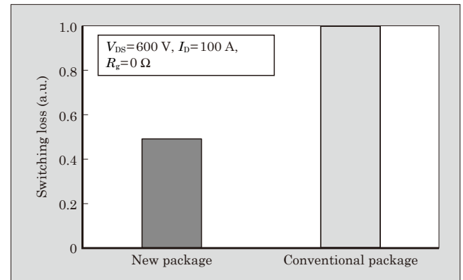
Fig.4 Switching loss of modules with SiC devices
