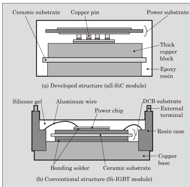
Fig.1 Cross-sectional views of modules
