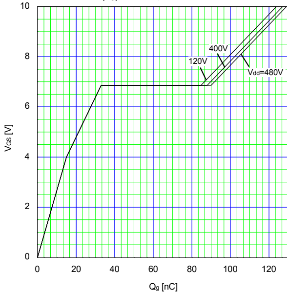
Typical Gate Charge Characteristics V_{GS}=f(Q_g): I_D=47\text{A}, T_{ch}=25^\circ\text{C}
