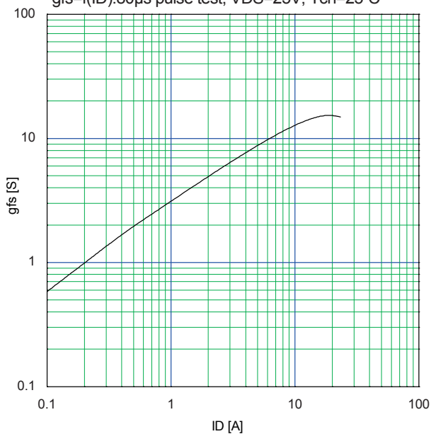
Typical Transconductance
