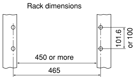
Slide rail mounting method
