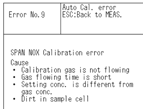
Display of error contents
