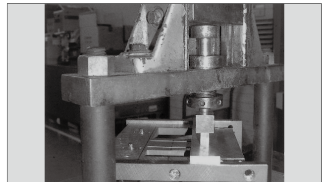
Fig.6 Component impact strength test conditions
