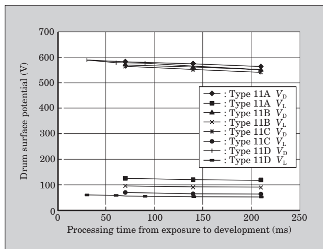
Fig.10 Photo response of positively charged OPCs
