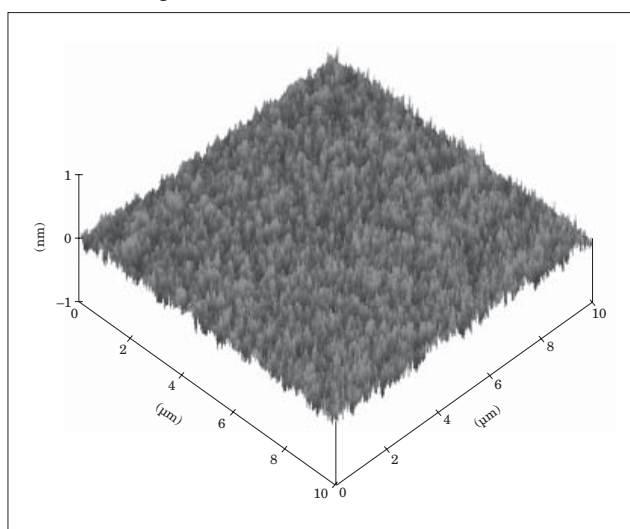
Fig.5 Surface profile of substrate for perpendicular magnetic recording media
