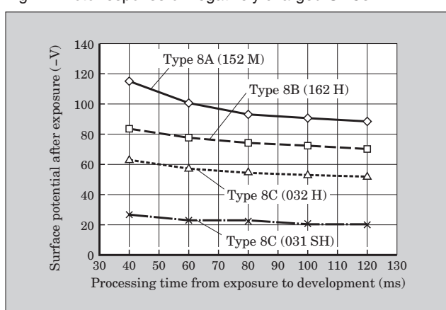
Fig.7 Photo response of negatively charged OPCs
