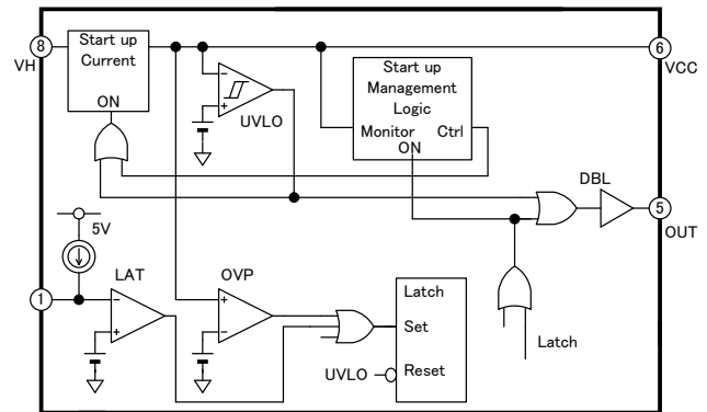
Fig. 12 Overvoltage protection circuit
