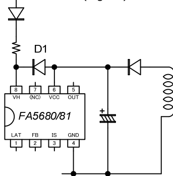
Fig. 32 Prevention of negative voltage applied to VH pin
