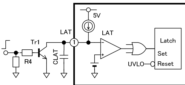
Fig. 22 Latch cutoff function by external signal
