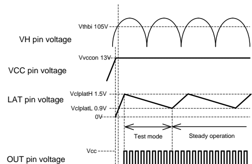
LATCH operation at start-up
