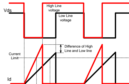
Fig.20 Overload detection level on input voltage (1)
