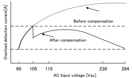
Fig.20 Overload detection level on input voltage (2)
