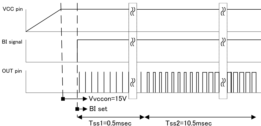
Fig.9.Soft-start function
