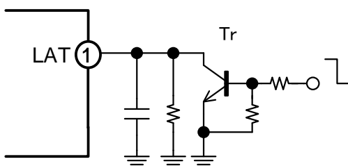
Fig.13 Latch circuit by external signal
