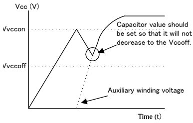
Fig.26 VCC pin voltage at start-up
