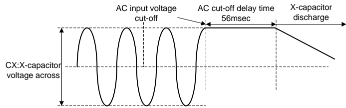
Fig11.X-Capacitor discharge operation
