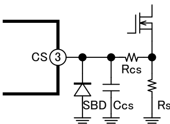
Fig.35 inhibit CS pin from minus voltage
