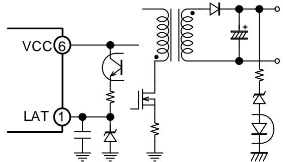
Fig.15 Over voltage circuit (2)
