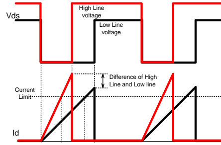
Fig.19 Overload detection level on input voltage (1)
