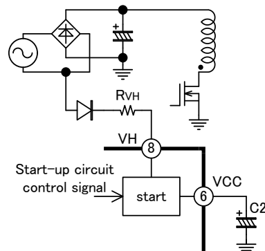
Fig.32 VH pin circuit (2)
