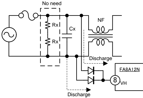
Fig10. VH pin discharge circuit
