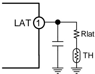
Fig.12 Over temperature circuit
