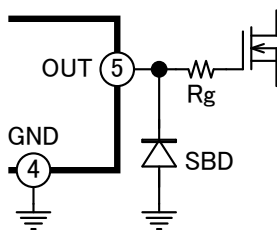
Fig.34 inhibit OUT pin from minus voltage
