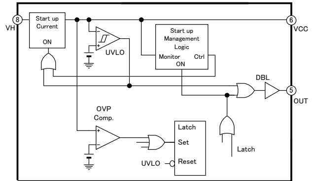
Fig.29 Over voltage circuit block
