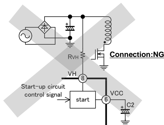
Fig.33 VH pin circuit (3)
