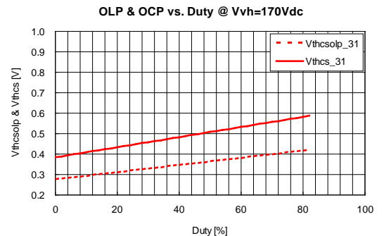
Fig.21 OLP,OCP CS threshold voltage vs. Duty
