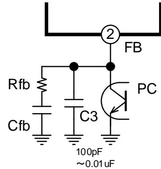
Fig.16 FB pin circuit
