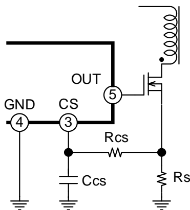
Fig.18 CS pin filter
