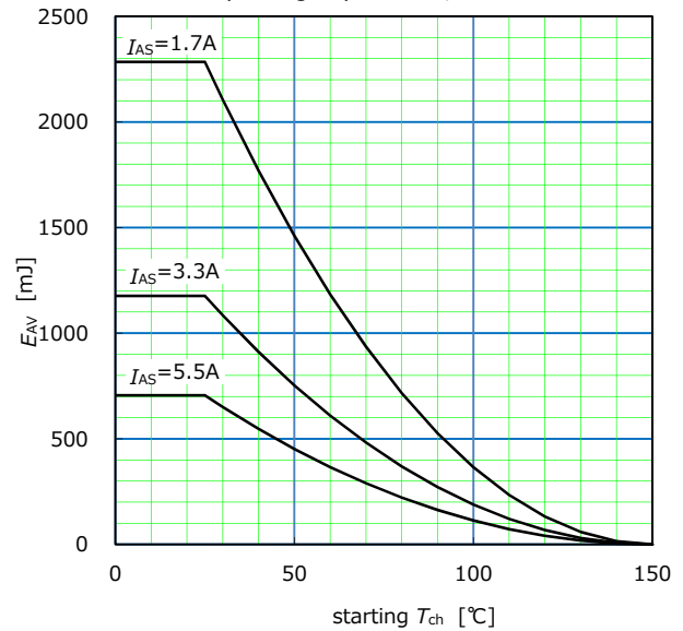
Maximum Avalanche Energy vs. starting T_{ch} E_{(AV)}=f(\text{starting } T_{ch}): V_{CC}=60V, I_{(AV)} \leq 5.5A
