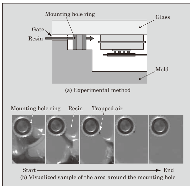
Fig. 6 Experiment of resin flow visualization
