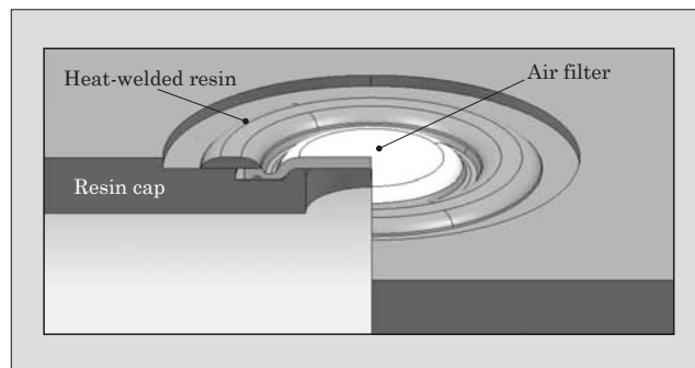
Fig.7 Cross-sectional view of air filter mounting part
