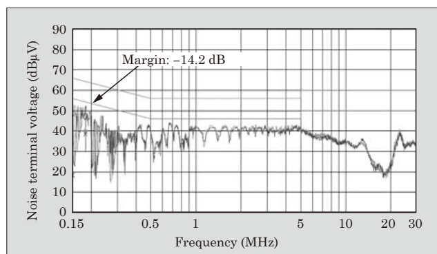
Fig. 9 Evaluation results for power supply conduction noise
