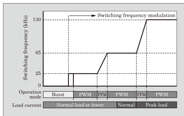
Fig. 3 3-stage switching frequency characteristics
