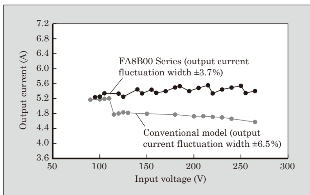
Fig. 4 Comparison of output current during overload
