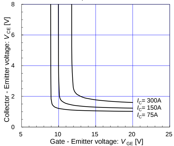
Collector-Emittor voltage vs. Gate-Emittor voltage (typ.) T_{vj} = 25^{\circ}\text{C} / chip
