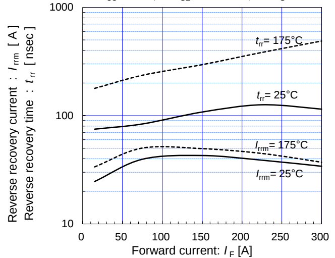
Reverse recovery characteristics (typ.) V_{CC} = 300V , V_{GE} = +15/-15V , R_G = 18\Omega
