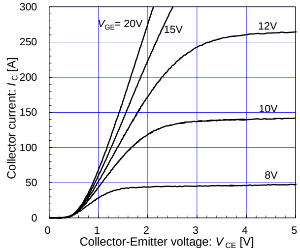
Collector current vs. Collector-Emittor voltage (typ.) T_{vj} = 175^{\circ}\text{C} / chip
