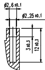
Section A-A Weight: 310 g (typ.)
