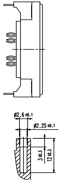
Section A-A Weight: 310 g (typ.)
