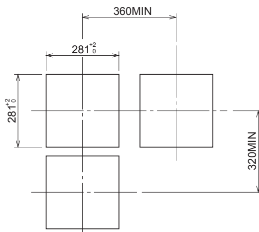
Panel cut dimensions (unit: mm)
