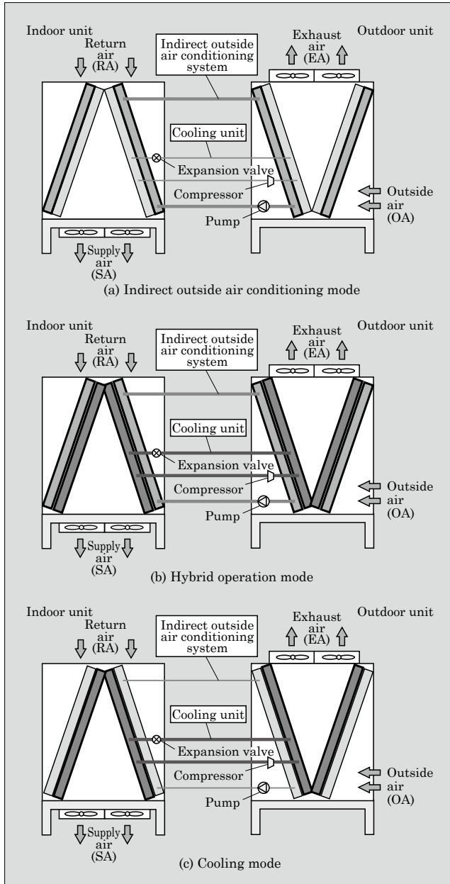
Fig.4 Operation of major equipment at each cooling mode
