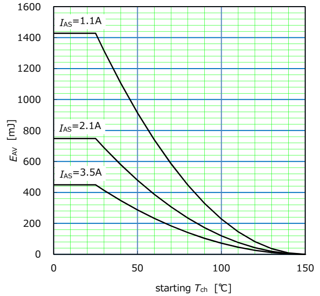
Maximum Avalanche Energy vs. starting T_{ch} E_{(AV)}=f(\text{starting } T_{ch}): V_{CC}=60\text{V}, I_{(AV)} < 3.5\text{A}
