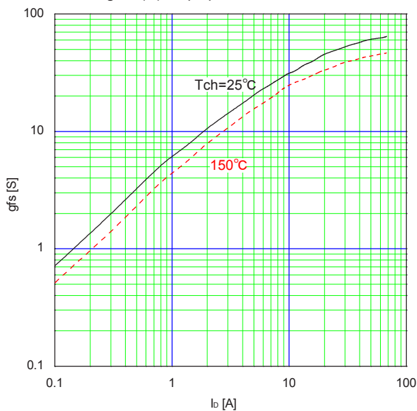
Typical Transconductance g_{fs}=f(I_D) : 80μs pulse test, V_{DS}=25V
