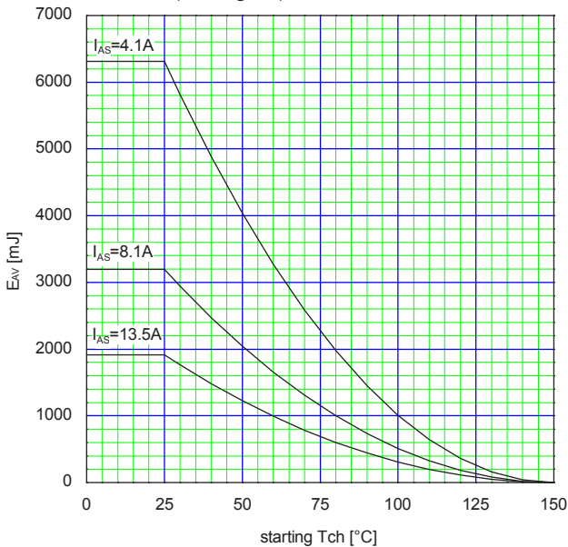
Maximum Avalanche Energy vs. starting T_{ch} E_{(AV)}=f(\text{starting } T_{ch}): V_{CC}=60V, I_{(AV)} \le 13.5A
