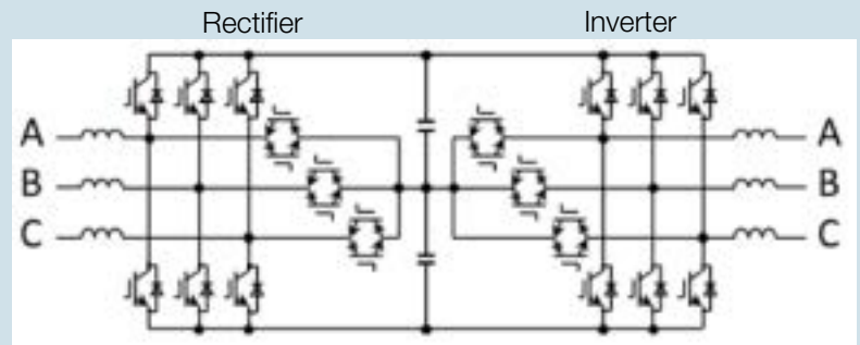
Use of RB-IGBT's reduces parts count and switching losses
