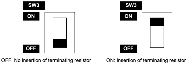
Figure 2.3 Terminating Resistor Switch Settings
