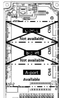
Figure 3.1 In the case of FRENIC-MEGA series
