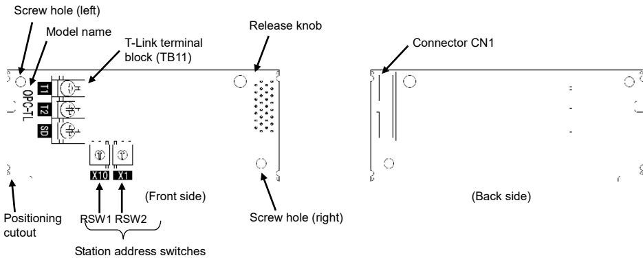
Figure 2.1 Names of Parts on T-Link Communications Card
