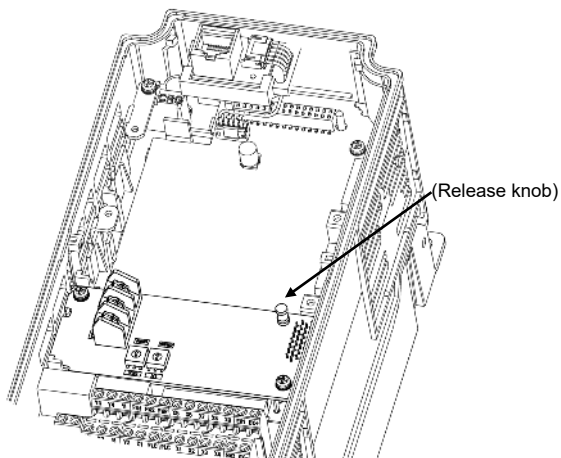
Figure 3.3 Mounting Completed
