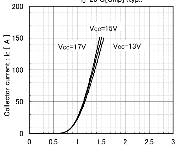
Collector current vs. Collector–Emitter voltage T_j=25^\circ\text{C} [Chip] (typ.)
