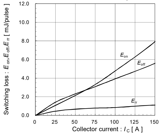
Switching loss vs. Collector current (typ.) V_{DC}=300\text{V}, V_{CC}=15\text{V}, T_{vj}=125^\circ\text{C}
