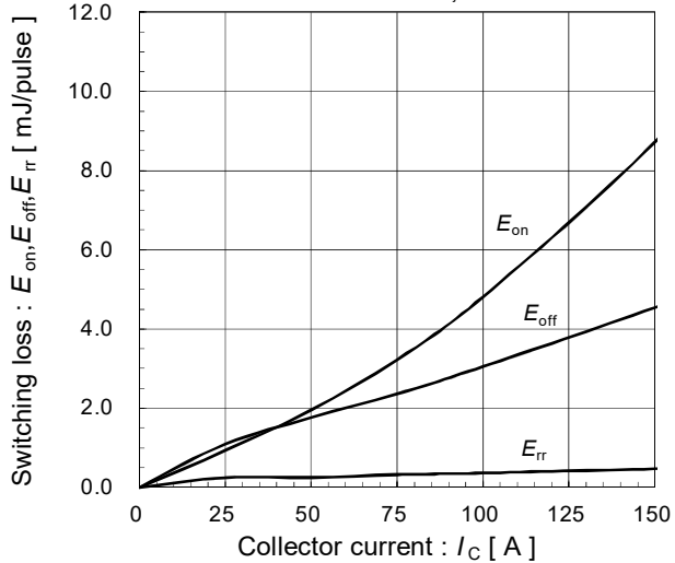
Switching loss vs. Collector current (typ.) V_{DC}=300\text{V}, V_{CC}=15\text{V}, T_{vj}=25^\circ\text{C}
