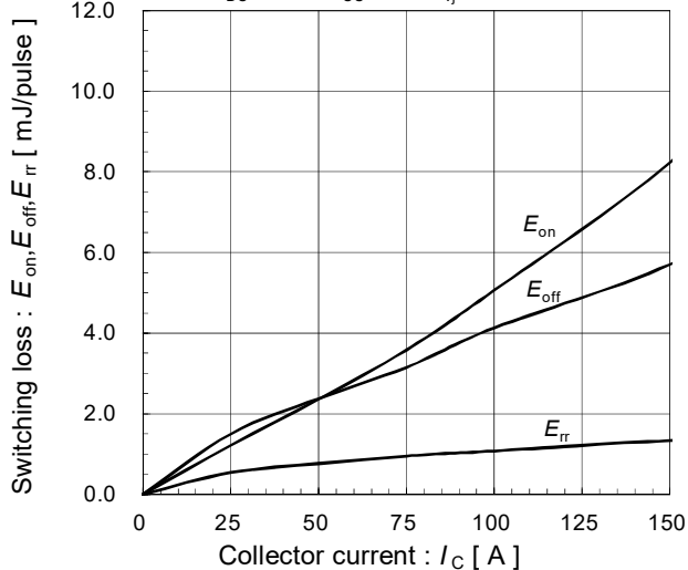
Switching loss vs. Collector current (typ.) V_{DC}=300\text{V}, V_{CC}=15\text{V}, T_{vj}=150^\circ\text{C}
