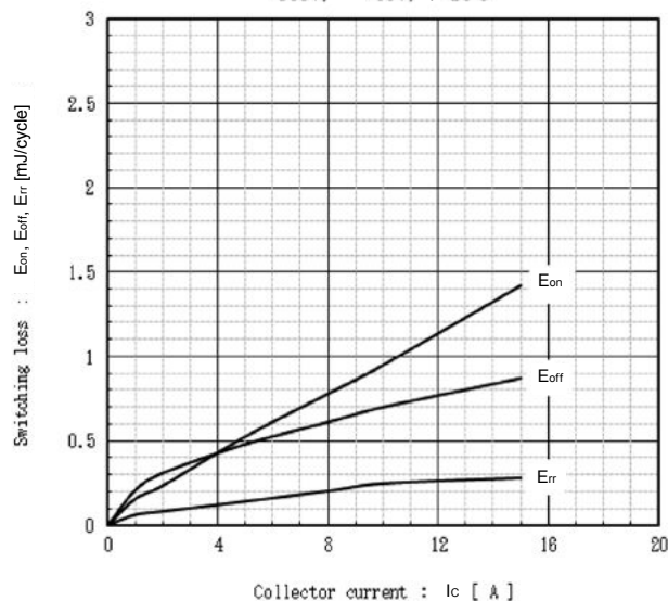
Switching Loss vs. Collector Current (typ.) V_{cc}=600V, V_{ce}=15V, T_j=25^{\circ}C
