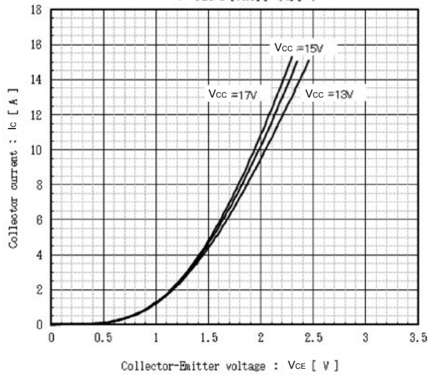
Collector current vs. Collector-Emmitter voltage T_J = 125^\circ\text{C} [Chip] (typ.)
