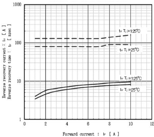
Reverse recovery characteristics (typ.) t_{rr}, I_{rr} vs. If V_{DC} = 600V, V_{CC} = 15V
