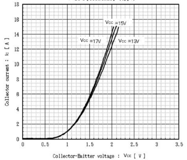
Collector current vs. Collector-Emmitter voltage T_J = 25^\circ\text{C} [Terminal] (typ.)
