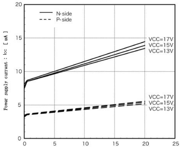
Power supply current vs. Switching frequency T_J = 25^\circ\text{C} (\text{typ.})
