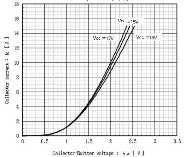
Collector current vs. Collector-Emmitter voltage T_J = 125^\circ\text{C} [Terminal] (typ.)
