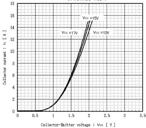
Collector current vs. Collector-Emmitter voltage T_J = 25^\circ\text{C} [Chip] (typ.)
