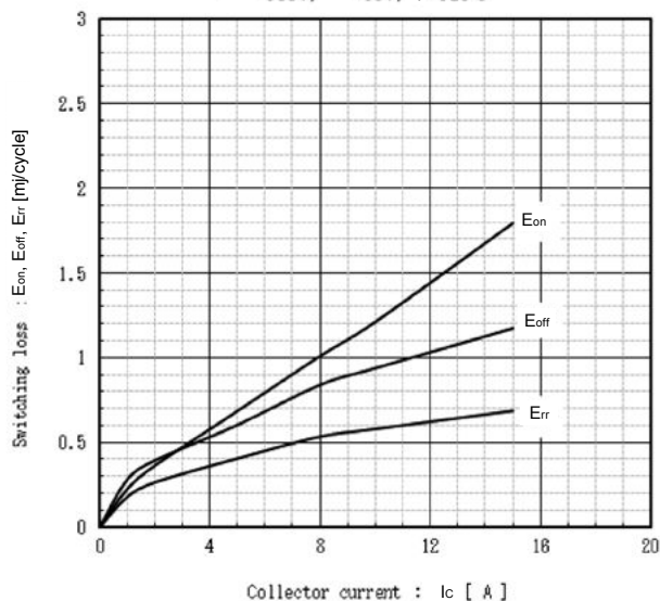
Switching Loss vs. Collector Current (typ.) V_{cc}=600V, V_{ce}=15V, T_j=125^{\circ}C
