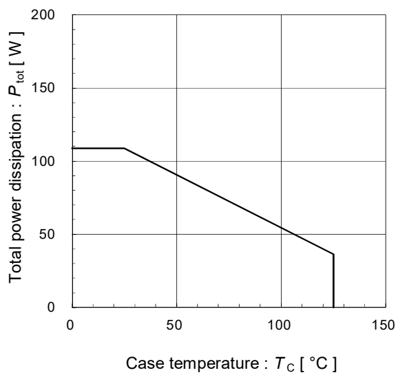
Power derating for RC-IGBT (max.) [ per device ]
