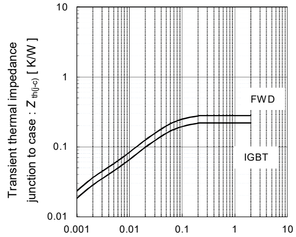
Transient thermal resistance (max.)
