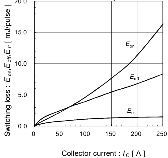
Switching loss vs. collector current (typ.) V_{DC}=300\text{V}, V_{CC}=15\text{V}, T_{vj}=125^\circ\text{C}
