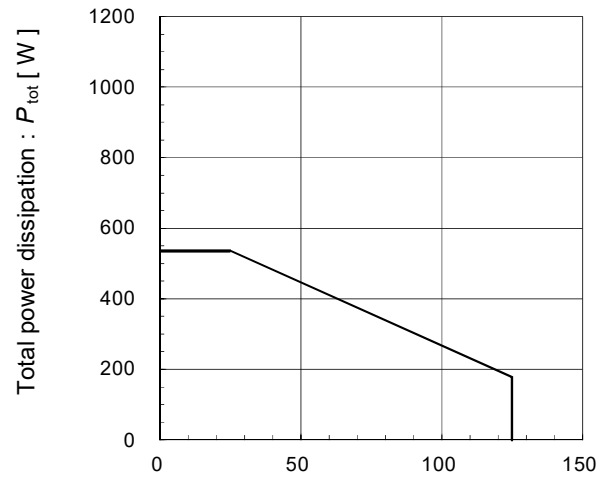
Power derating for FWD (max.) [per device]
