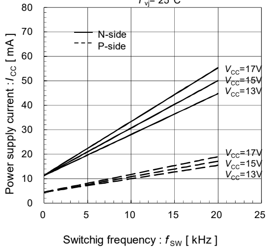
Power supply current vs. Switching frequency (typ.) T_{vj} = 25^\circ\text{C}
