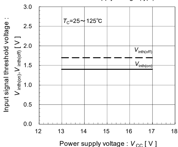
Input signal threshold voltage
