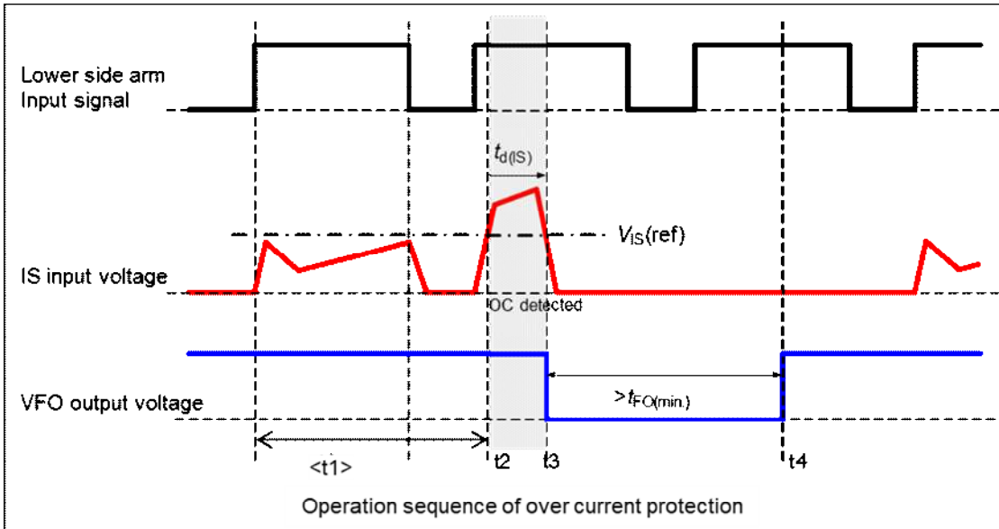
Fig.2-2_Operation_sequence_of over_current_protection
