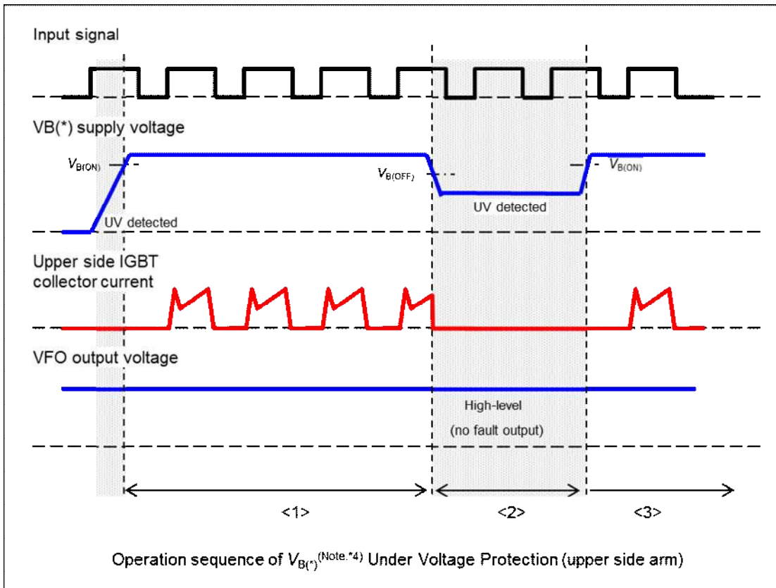
Fig.2-5 Operation sequence of V_{B(*)} under voltage protection (upper side arm)
