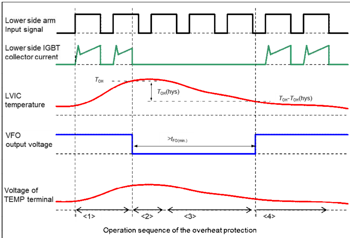
Fig.2-6 Overheat protection
