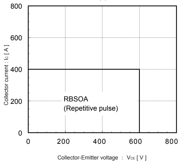
Reversed biased safe operating area V_{CE}=15V, T_J \leq 125^\circ C
