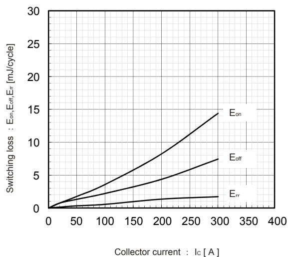
Switching Loss vs. Collector Current (typ.) V_{DC}=300V, V_{CE}=15V, T_J=25^\circ C
